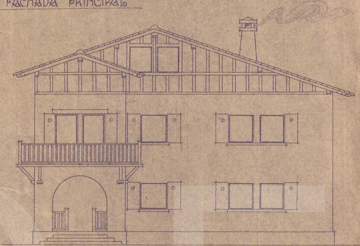
FACHADA PRINCIPAL
